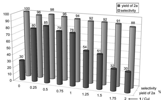
Figure 2. Effect of the 1 -to-CuI ratio on the yield of diaryl ether after 24 hours at 80 °C in acetonitrile.
