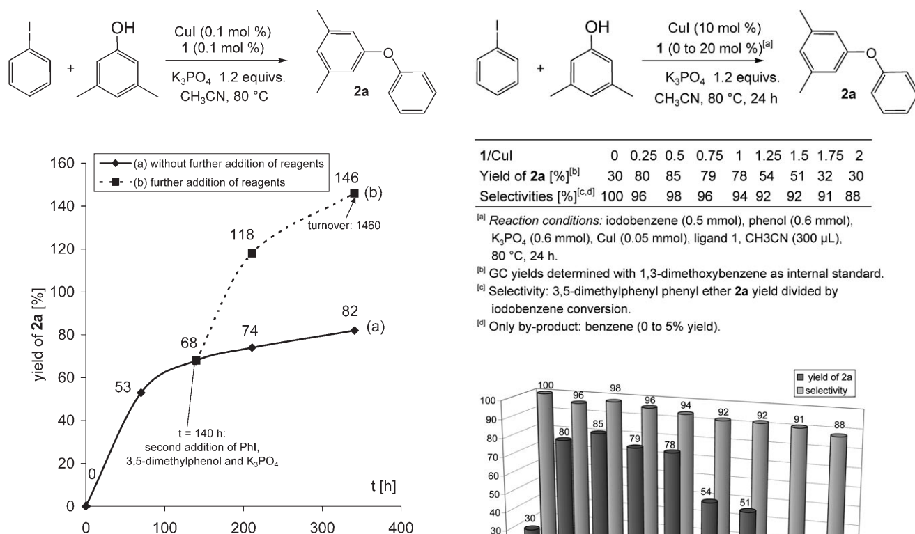
Figure 1. Coupling reaction of iodobenzene and 3,5-dimethylphenol under the catalysis of 0.1 mol % of CuI and ligand 1 . Reaction conditions: (a) without further addition of reagents: iodobenzene (5 mmol), 3,5-dimethylphenol (6 mmol), base (6 mmol), CuI (0.005 mmol), ligand 1 (0.005 mmol), CH 3 CN (3 mL), 80 °C; (b) after 140 h at 80 °C, addition of iodobenzene (5 mmol), 3,5-dimethylphenol (5 mmol), base (5 mmol). GC yields determined with 1,3-dimethoxybenzene as internal standard. Solid line: without further addition of reagents; dashed line: with second addition of reagents.
